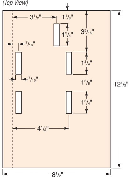
Jig (Top View)
