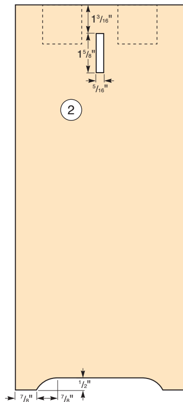
Leg (Front View)
