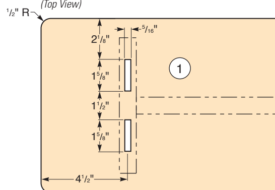
Top (Top View)
