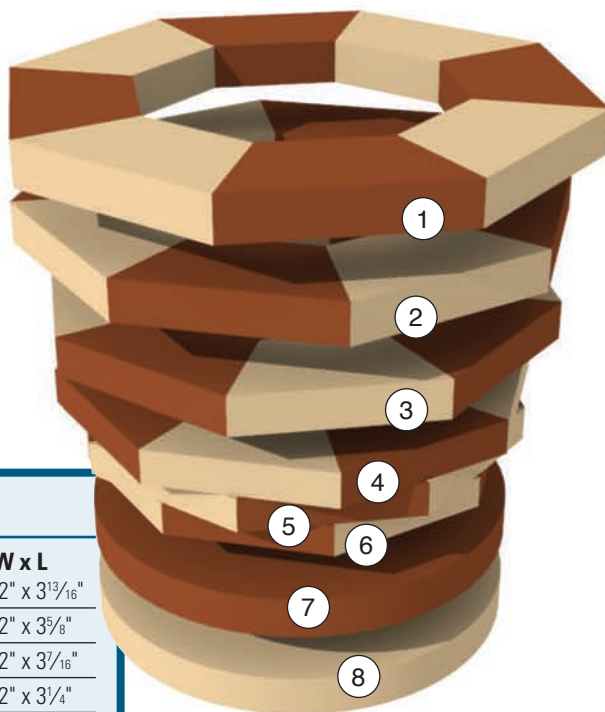
Exploded View
